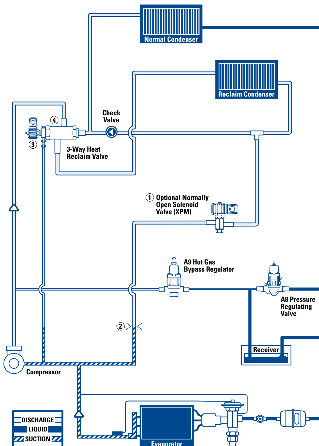
Series Condenser Typical Piping Schematic
